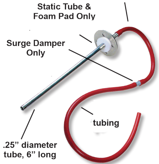
Static Pressure Probe Assembly
