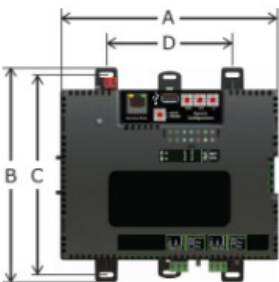
Figure 1: Physical Dimensions
