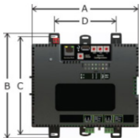
Figure 1: Physical Dimensions
