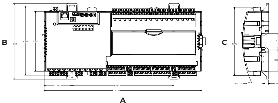
Figure 1: Physical Dimensions
