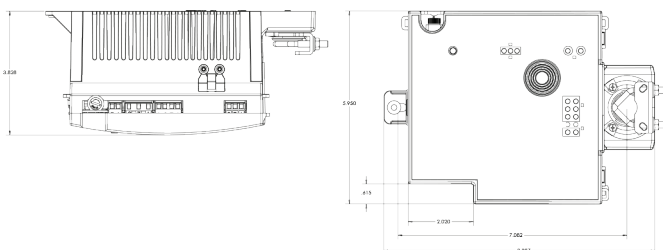
Figure 1: Physical Dimensions
