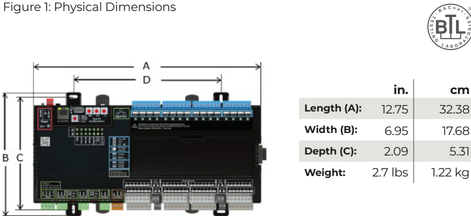
Figure 1: Physical Dimensions
