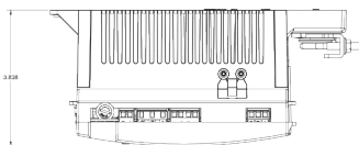
• Figure 1: Physical Dimensions
