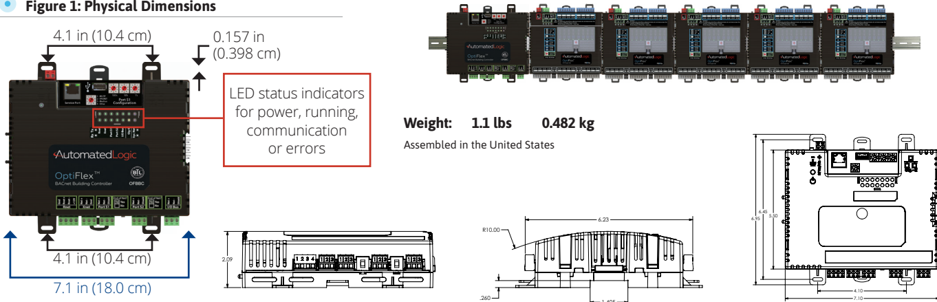
Figure 1: Physical Dimensions
